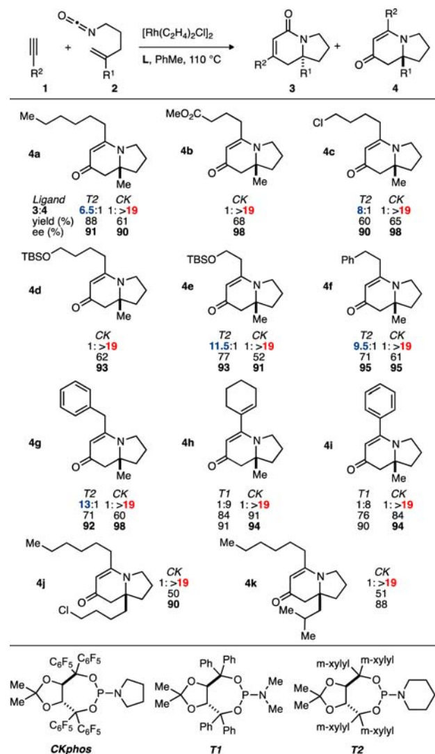
Figure 1. Isocyanate and alkyne substrate scope. Reaction conditions: 1, 2 (1.3 equiv), [Rh(C 2 H 4 ) 2 Cl] 2 (2.5 mol %), L (5 mol %) in PhMe at 110 °C for 16 h. The combined isolated yield is reported. The enantiomeric excess shown is of the major product. For T1 and T2, the results were previously reported; 4 2 equiv of 2 were used.
